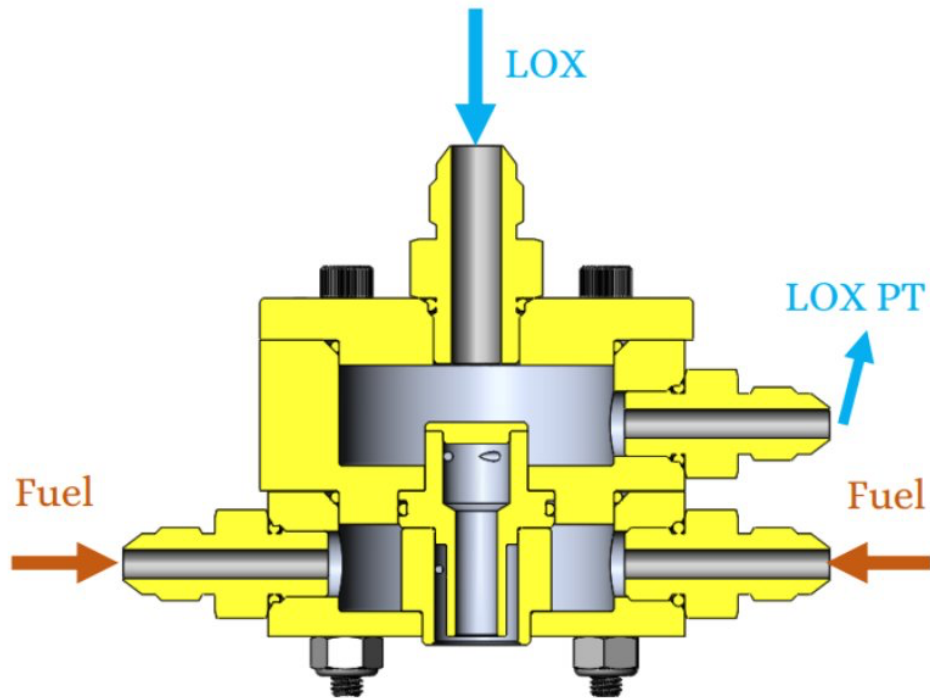
Fig. 2. Single element swirler assembly.
