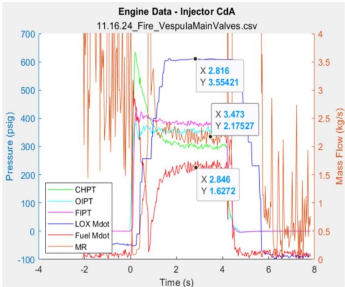
Fig. 16. Vespula injector hotfire data.
