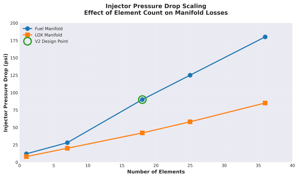
Figure 4.1. Injector Pressure Drop vs Element Count Scaling
