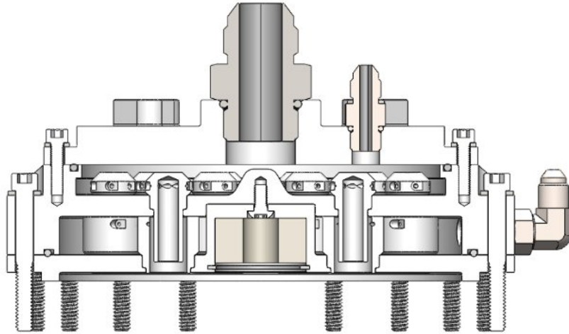
Fig. 12. Vespula injector CAD cross section
