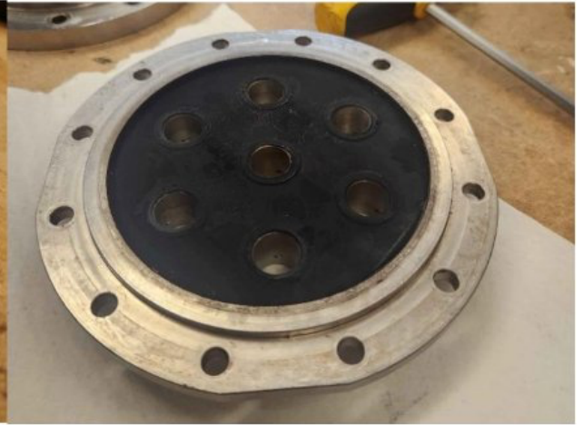
Fig. 11. Injector faceplate after hotfire
