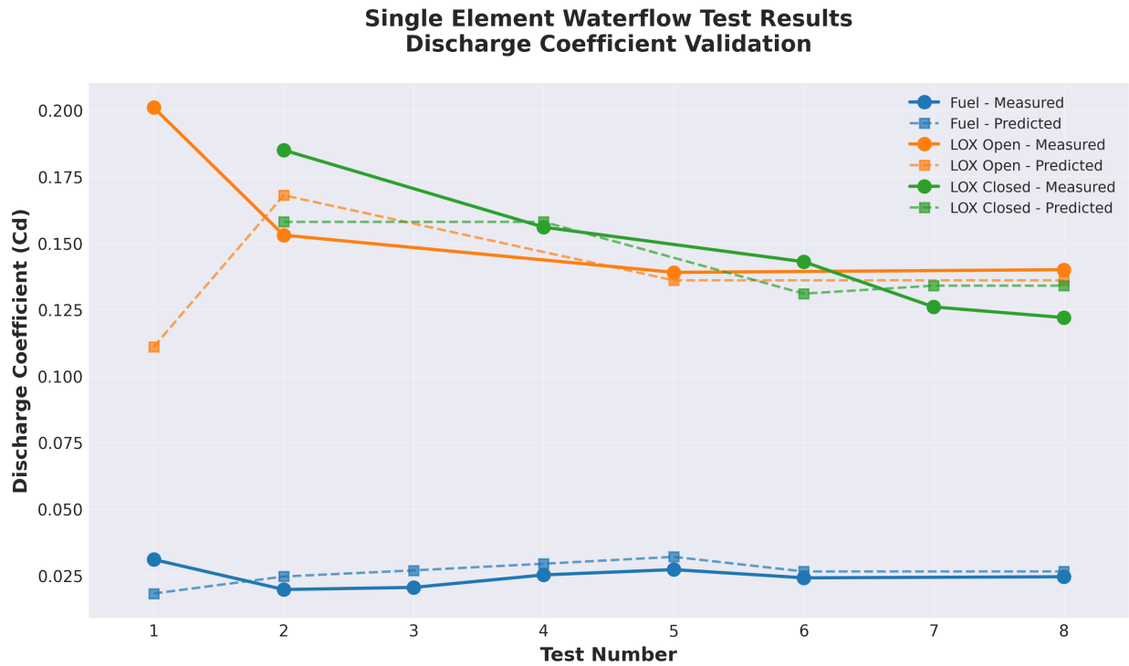
Figure 3.1. Single Element Waterflow Discharge Coefficient Validation
